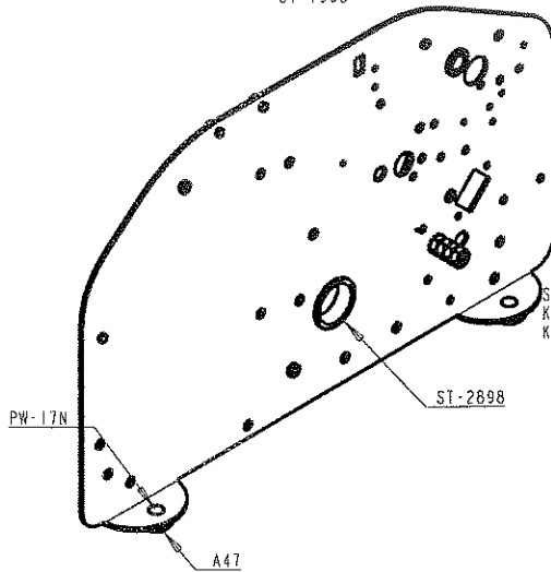
ITEM 1 - LEFT FRAME ASSY B500-L-XXX
