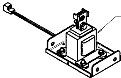
ITEM 3 - SOLENOID SHELF ASSY
