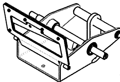
ITEM 31 E555-049-01 CUTTER YOKE ASSY
