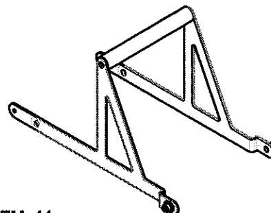
ITEM 14 E555-098-01 ASSY, LIFT ROLLER BRACKET
