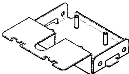
ITEM 30 E555-014-01 SOLENOID SHELF ASSY
